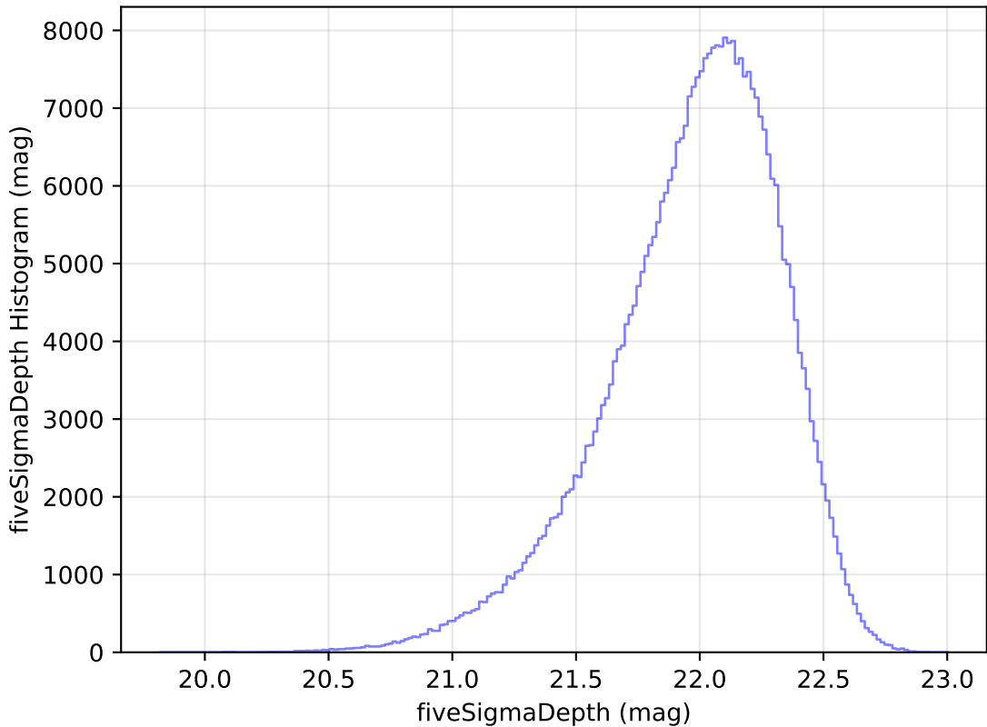
internal_u_expt30_nscale1.0v3.4_10yrs y: fiveSigmaDepth Histogram
