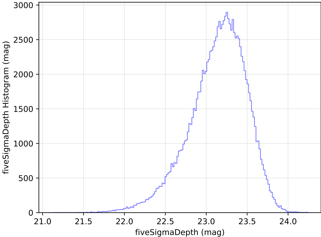
internal_u_expt30_nscale1.0v3.4_10yrs u: fiveSigmaDepth Histogram
