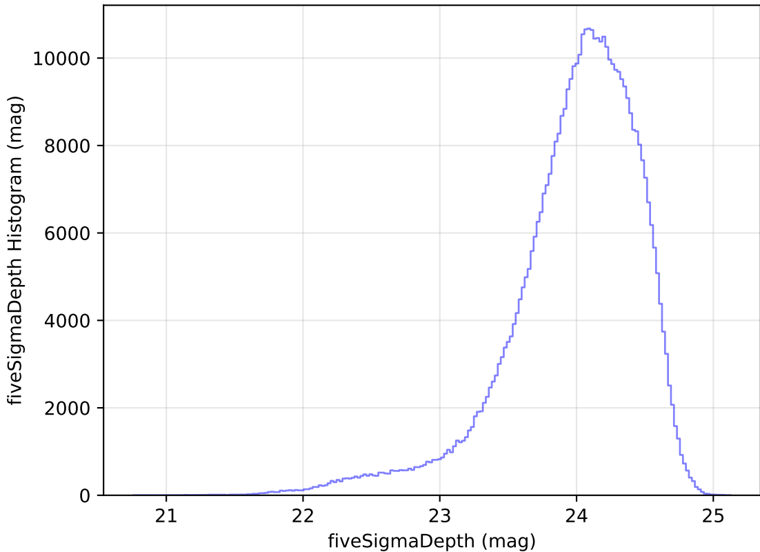
internal_u_expt30_nscale1.0v3.4_10yrs r: fiveSigmaDepth Histogram
