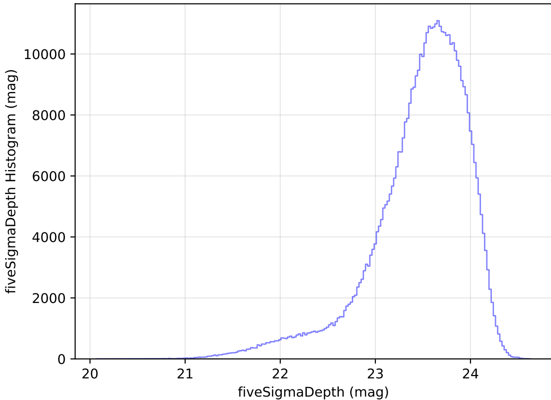
internal_u_expt30_nscale1.0v3.4_10yrs i: fiveSigmaDepth Histogram
