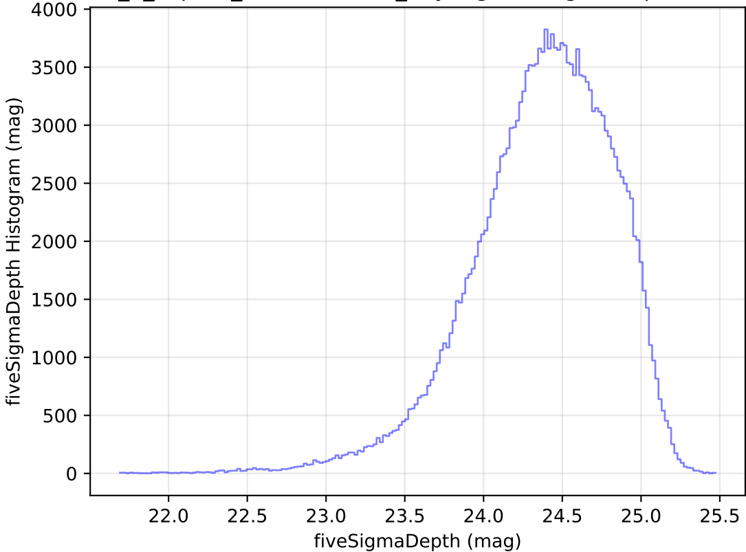
internal_u_expt30_nscale1.0v3.4_10yrs g: fiveSigmaDepth Histogram
