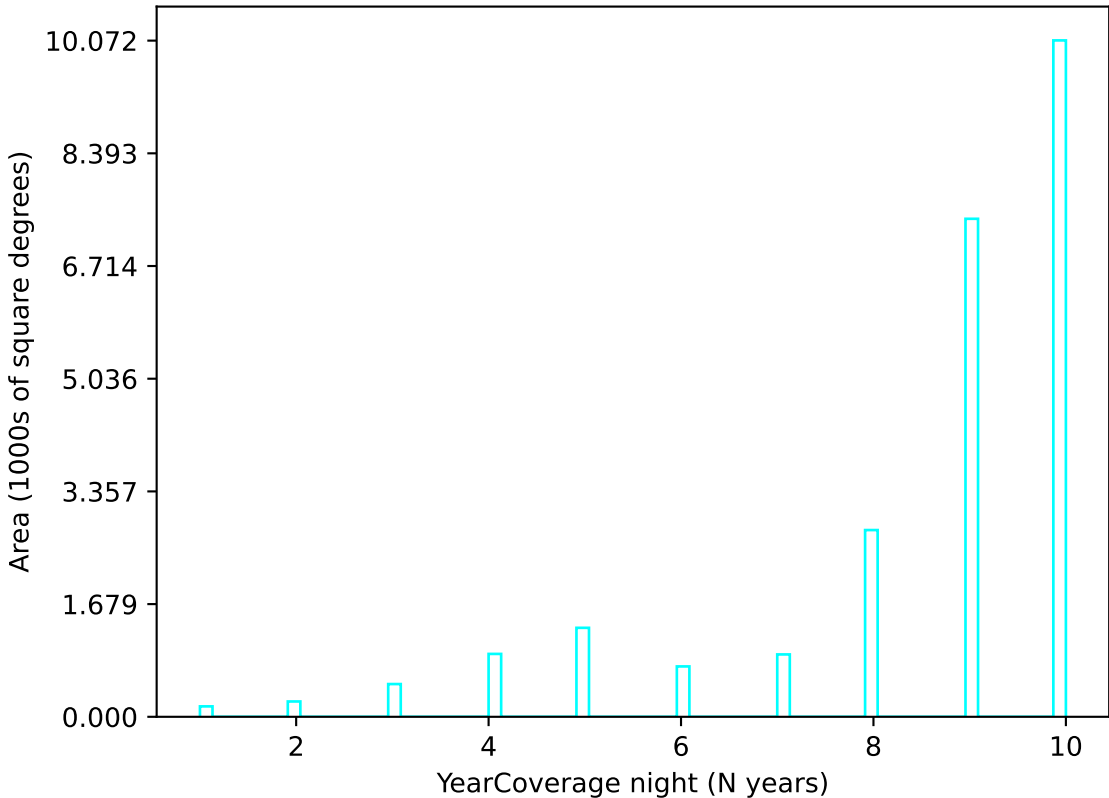
internal_u_expt30_nscale1.0v3.4_10yrs u band: YearCoverage night
