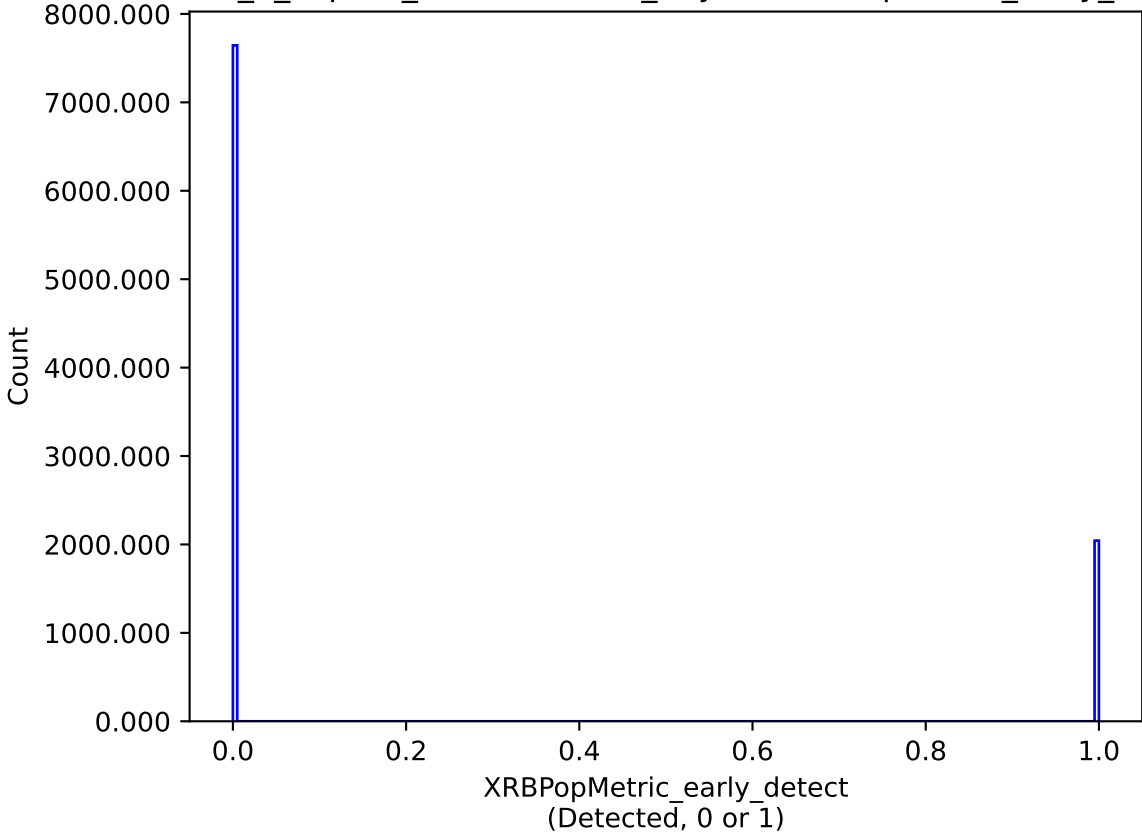
internal_u_expt30_nscale1.0v3.4_10yrs : XRBPoMetric_early_detect
