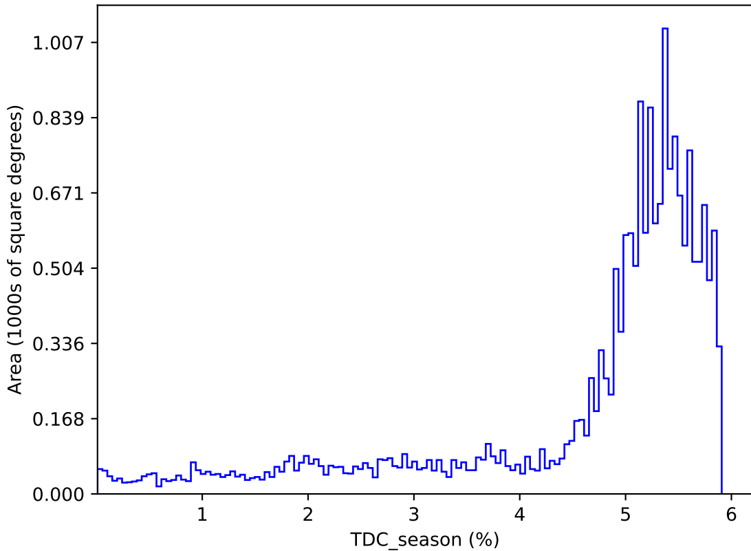
internal_u_expt30_nscale1.0v3.4_10yrs : TDC_season
