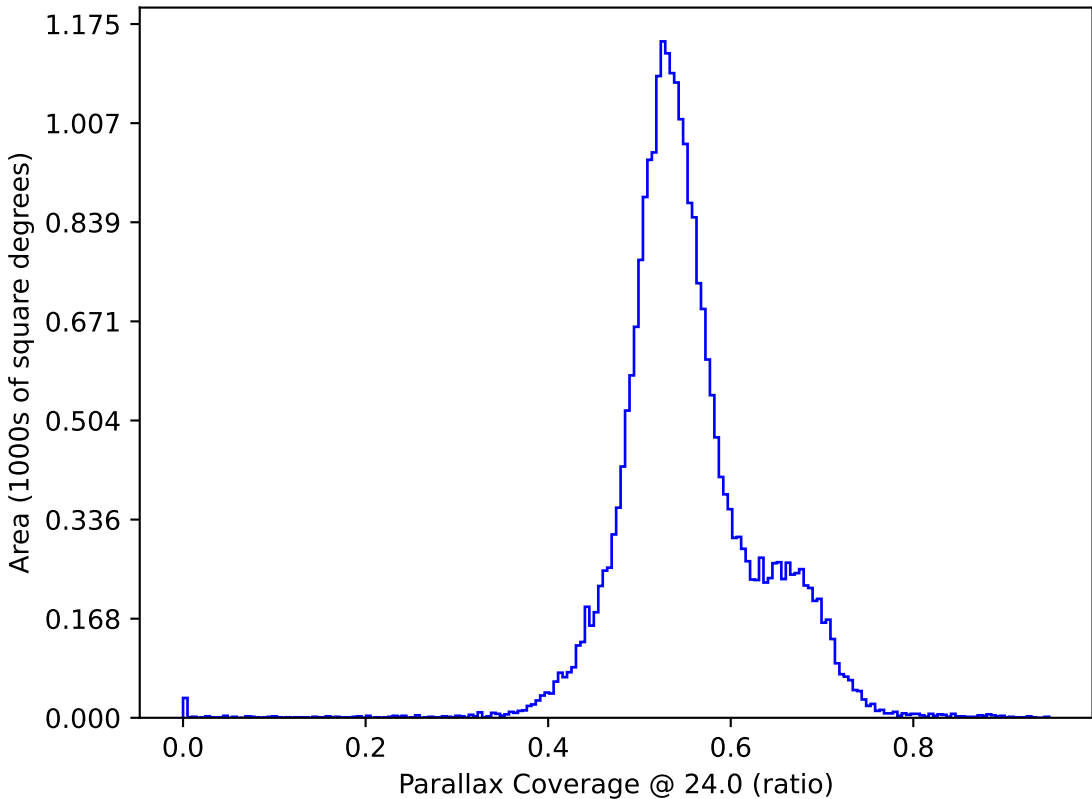
internal_u_expt30_nscale1.0v3.4_10yrs : Parallax Coverage @ 24.0
