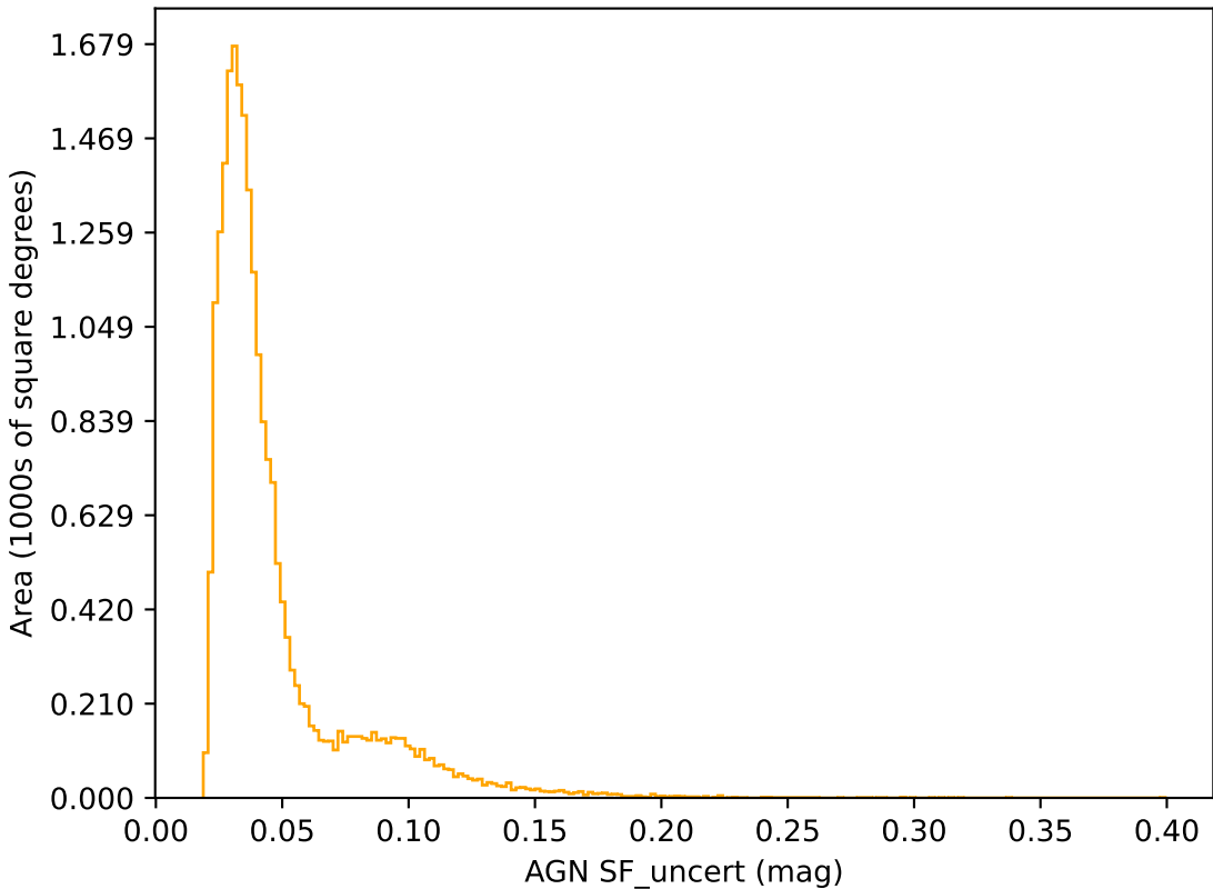
internal_u_expt30_nscale1.0v3.4_10yrs r band: AGN SF_uncert
