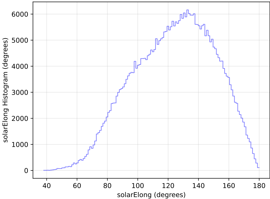
internal_u_expt30_nscale1.0v3.4_10yrs WFD y band: solarElong Histogram
