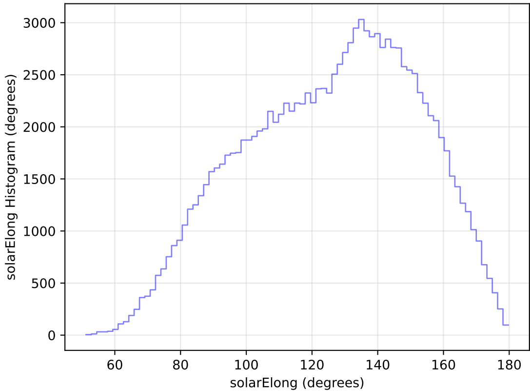
internal_u_expt30_nscale1.0v3.4_10yrs WFD u band: solarElong Histogram
