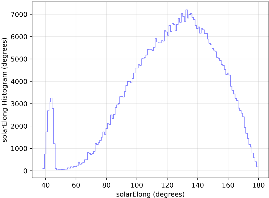
internal_u_expt30_nscale1.0v3.4_10yrs WFD r band: solarElong Histogram
