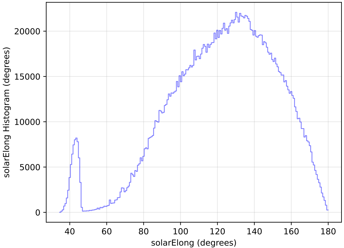
internal_u_expt30_nscale1.0v3.4_10yrs WFD all bands: solarElong Histogram
