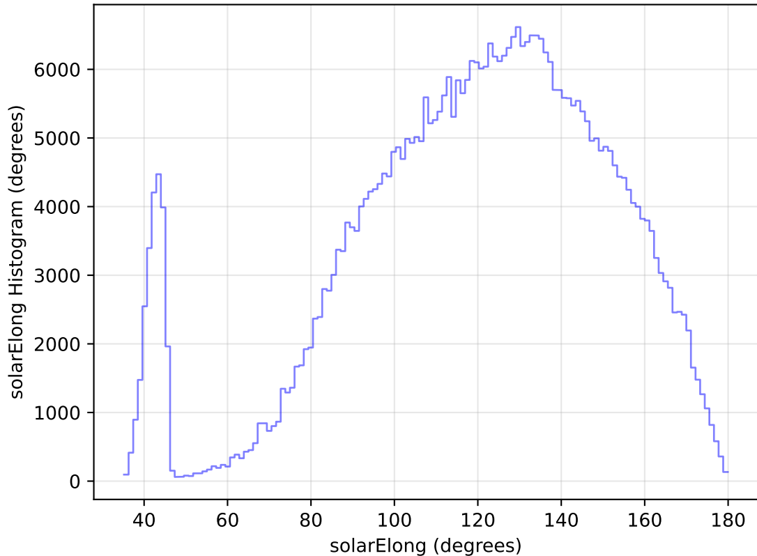
internal_u_expt30_nscale1.0v3.4_10yrs All sky z band: solarElong Histogram
