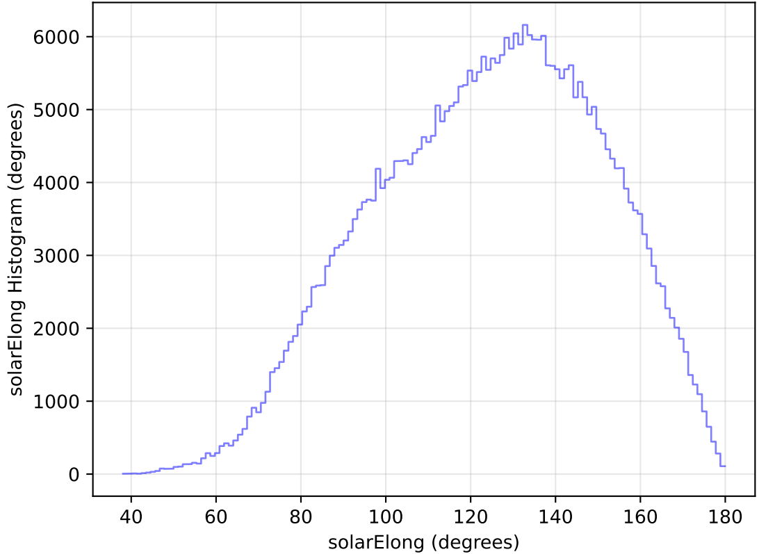
internal_u_expt30_nscale1.0v3.4_10yrs All sky y band: solarElong Histogram
