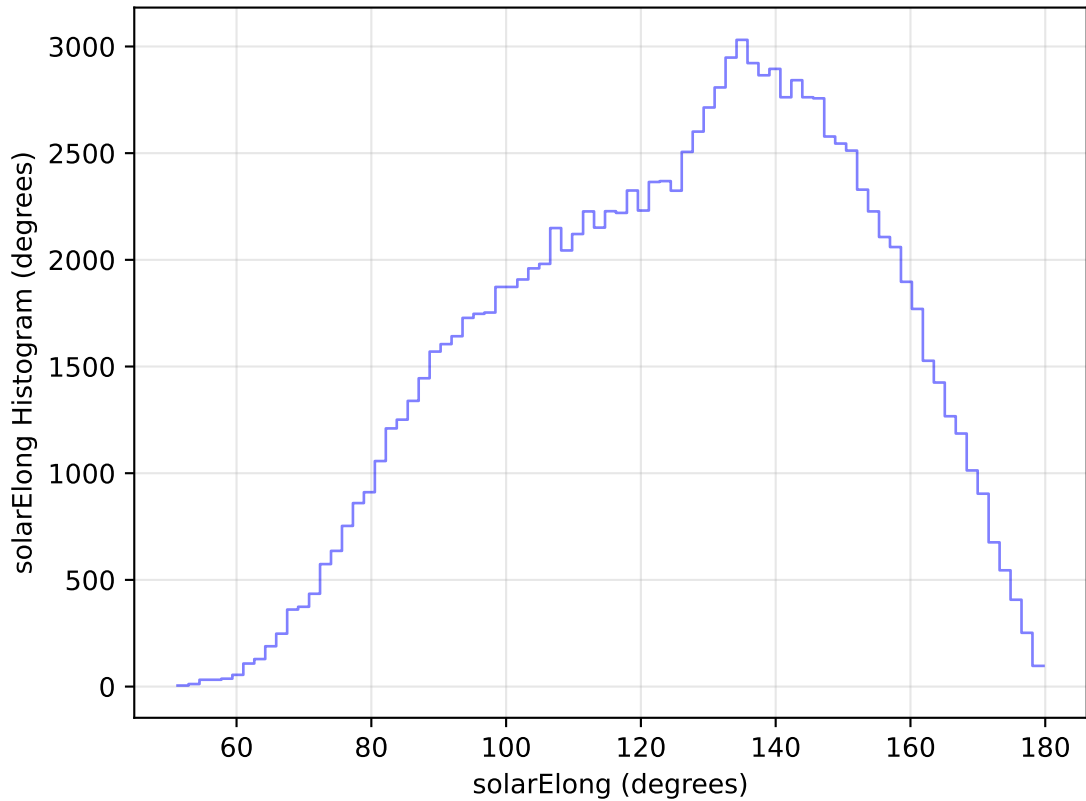
internal_u_expt30_nscale1.0v3.4_10yrs All sky u band: solarElong Histogram
