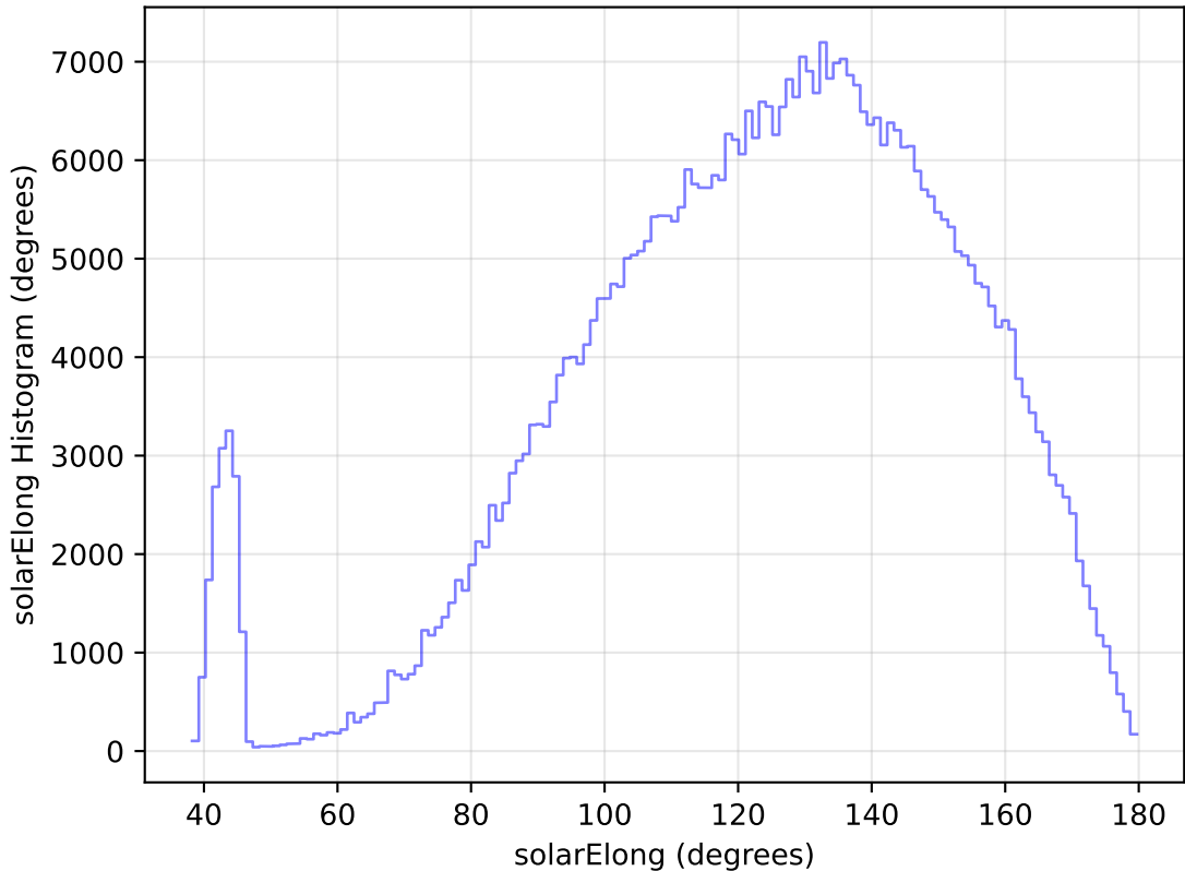
internal_u_expt30_nscale1.0v3.4_10yrs All sky r band: solarElong Histogram
