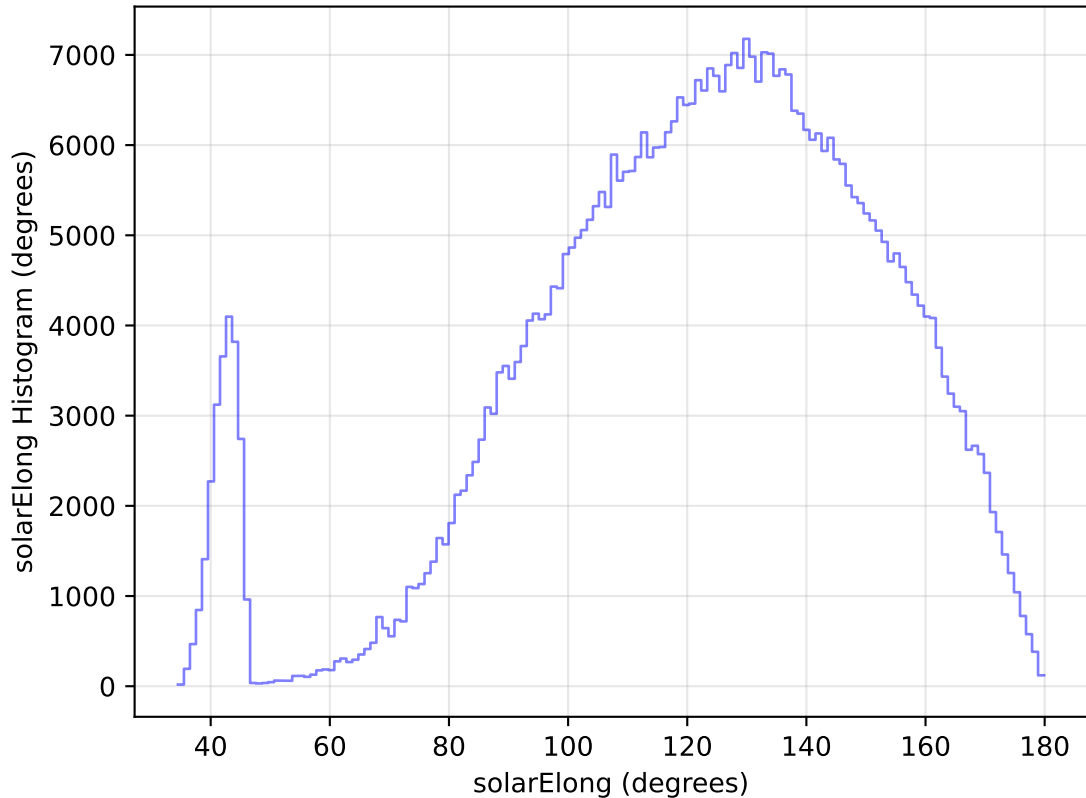
internal_u_expt30_nscale1.0v3.4_10yrs All sky i band: solarElong Histogram
