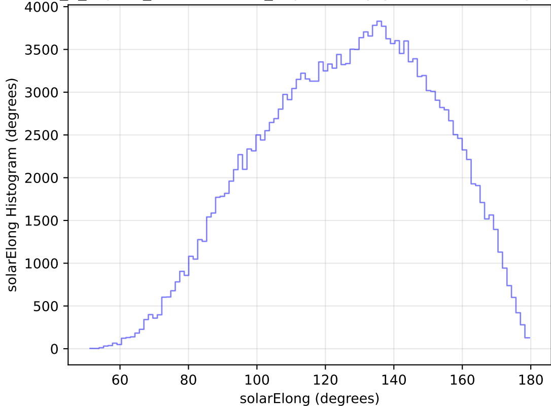
internal_u_expt30_nscale1.0v3.4_10yrs All sky g band: solarElong Histogram
