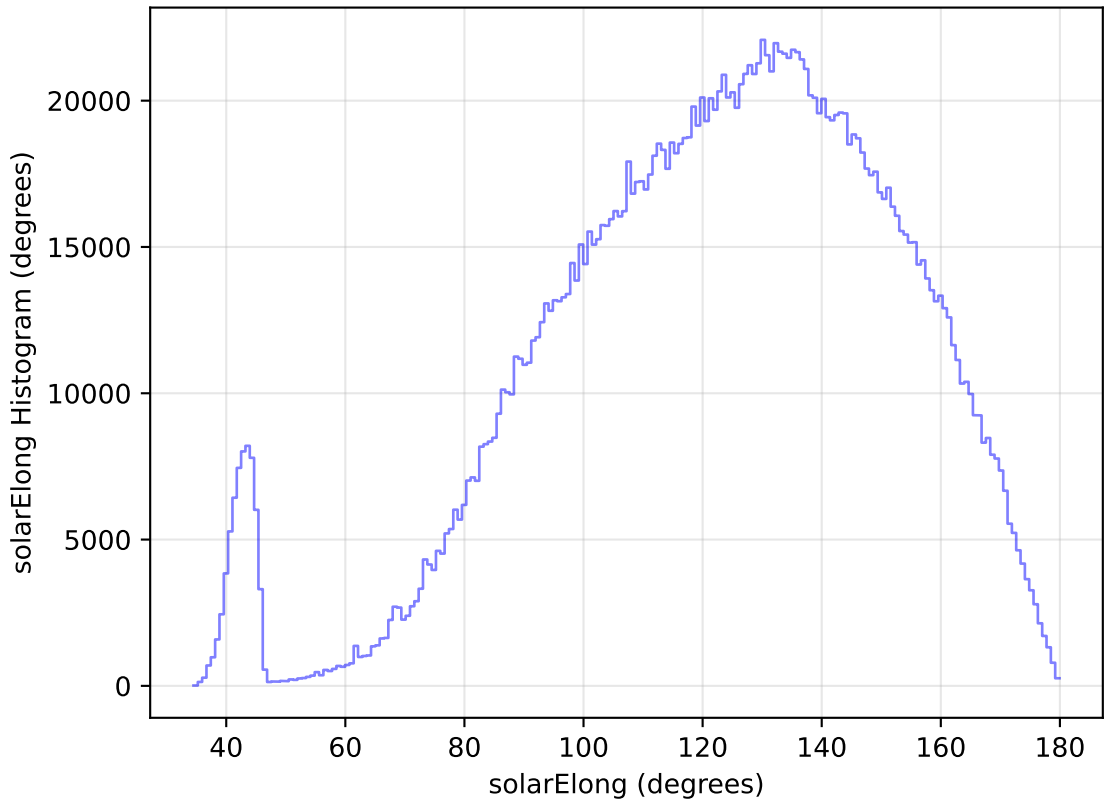
internal_u_expt30_nscale1.0v3.4_10yrs All sky all bands: solarElong Histogram
