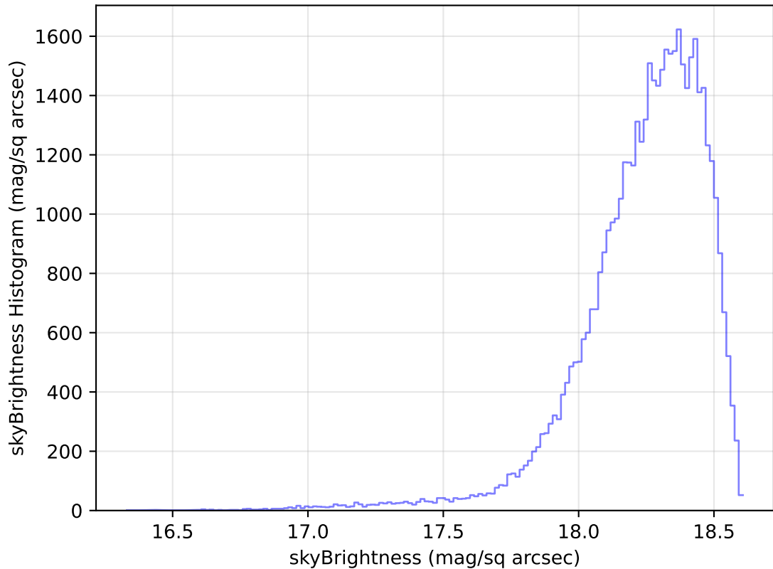
internal_u_expt30_nscale1.0v3.4_10yrs Yr 1 y band: skyBrightness Histogram
