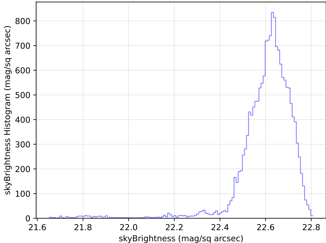
internal_u_expt30_nscale1.0v3.4_10yrs Yr 1 u band: skyBrightness Histogram
