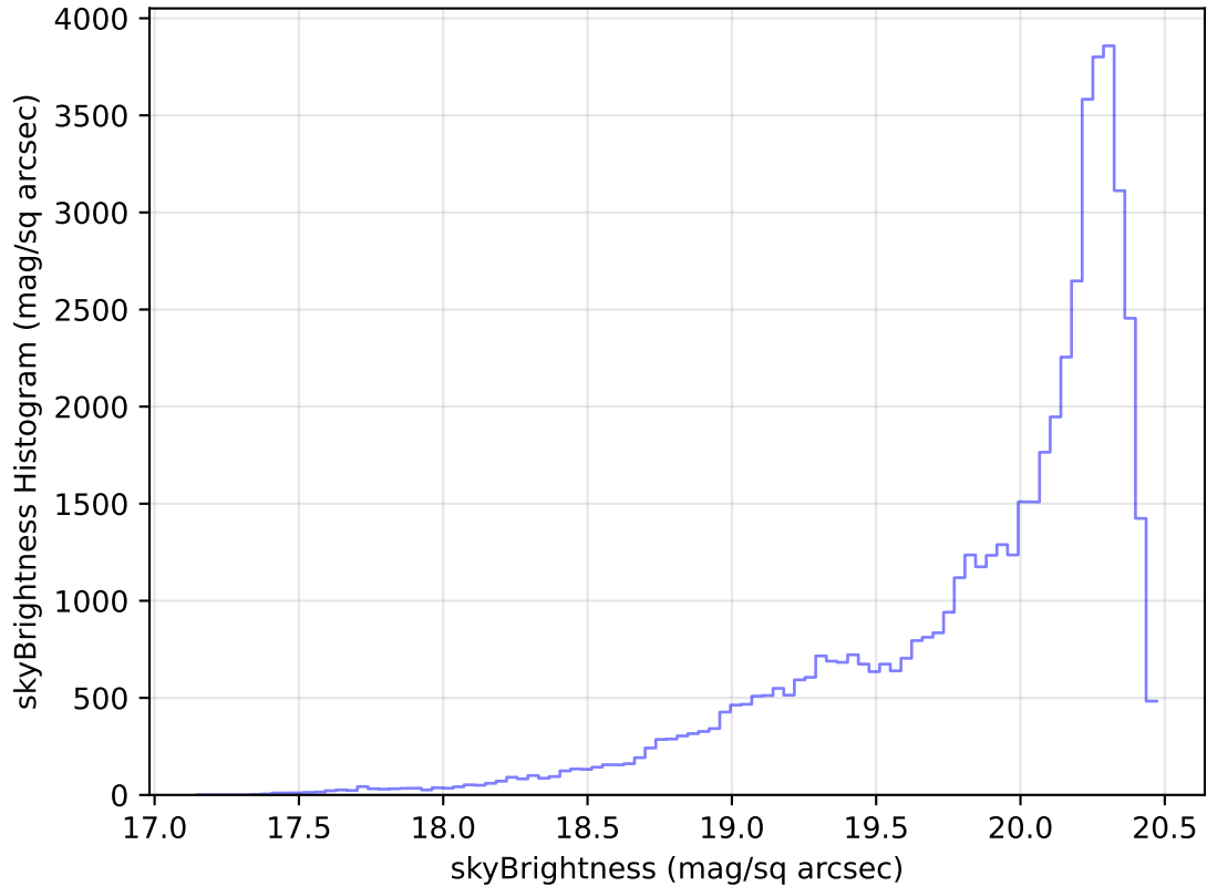
internal_u_expt30_nscale1.0v3.4_10yrs Yr 1 i band: skyBrightness Histogram
