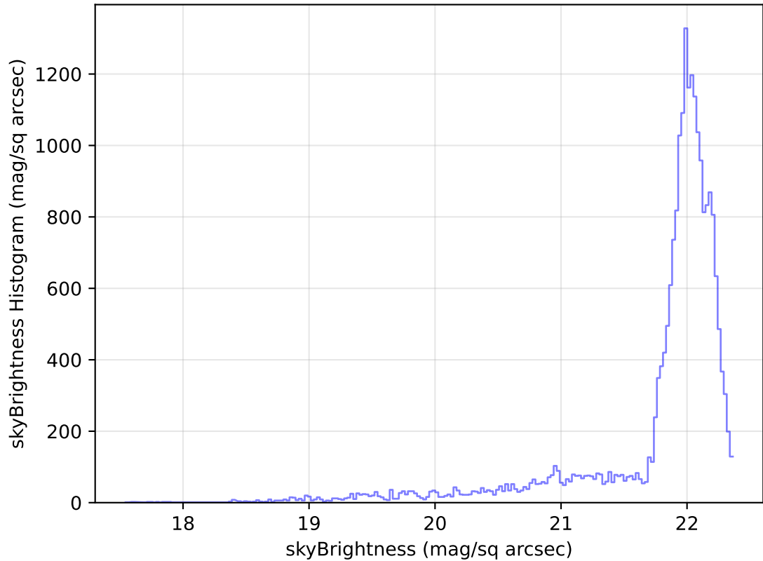
internal_u_expt30_nscale1.0v3.4_10yrs Yr 1 g band: skyBrightness Histogram
