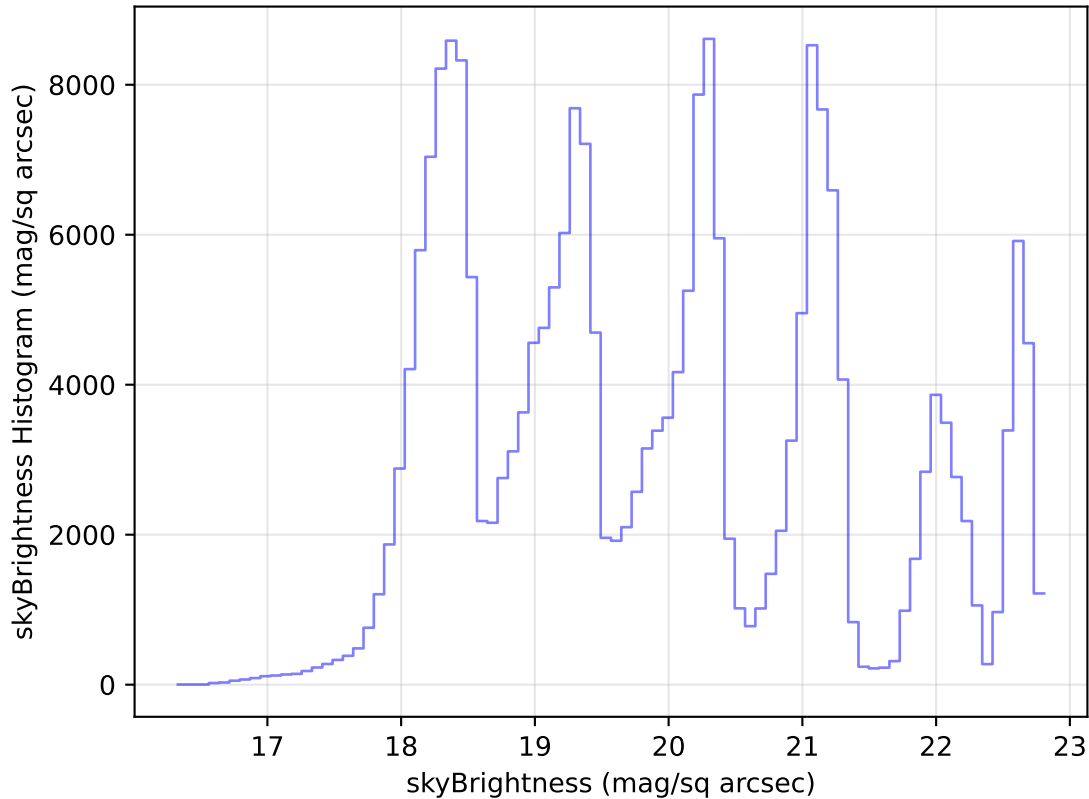
internal_u_expt30_nscale1.0v3.4_10yrs Yr 1 all bands: skyBrightness Histogram
