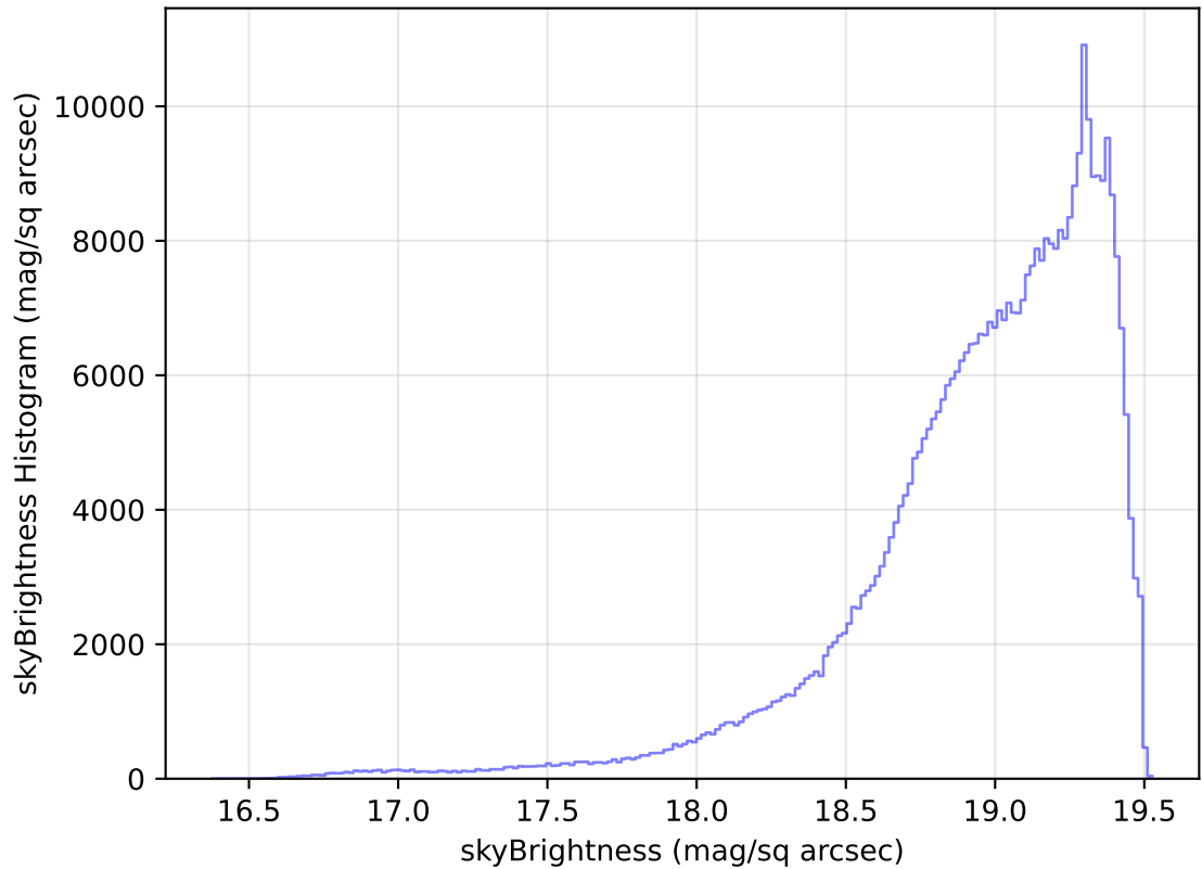
internal_u_expt30_nscale1.0v3.4_10yrs WFD z band: skyBrightness Histogram
