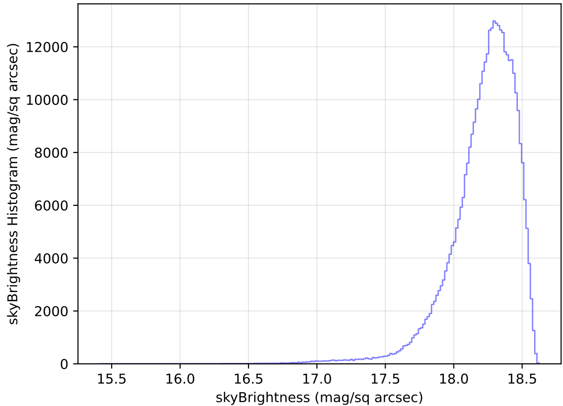
internal_u_expt30_nscale1.0v3.4_10yrs WFD y band: skyBrightness Histogram
