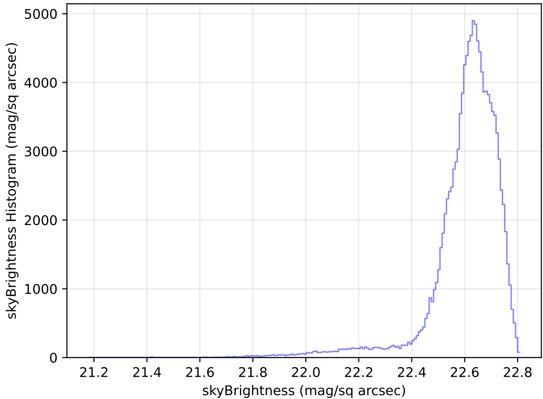
internal_u_expt30_nscale1.0v3.4_10yrs WFD u band: skyBrightness Histogram
