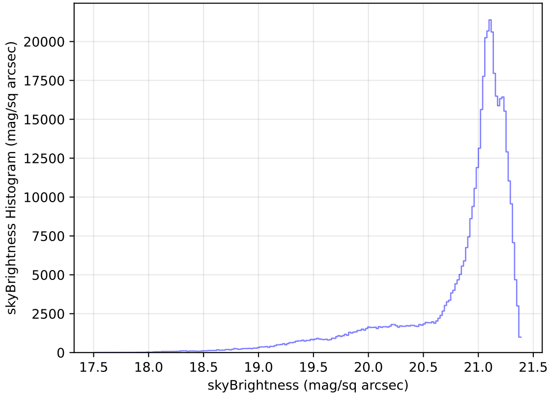
internal_u_expt30_nscale1.0v3.4_10yrs WFD r band: skyBrightness Histogram
