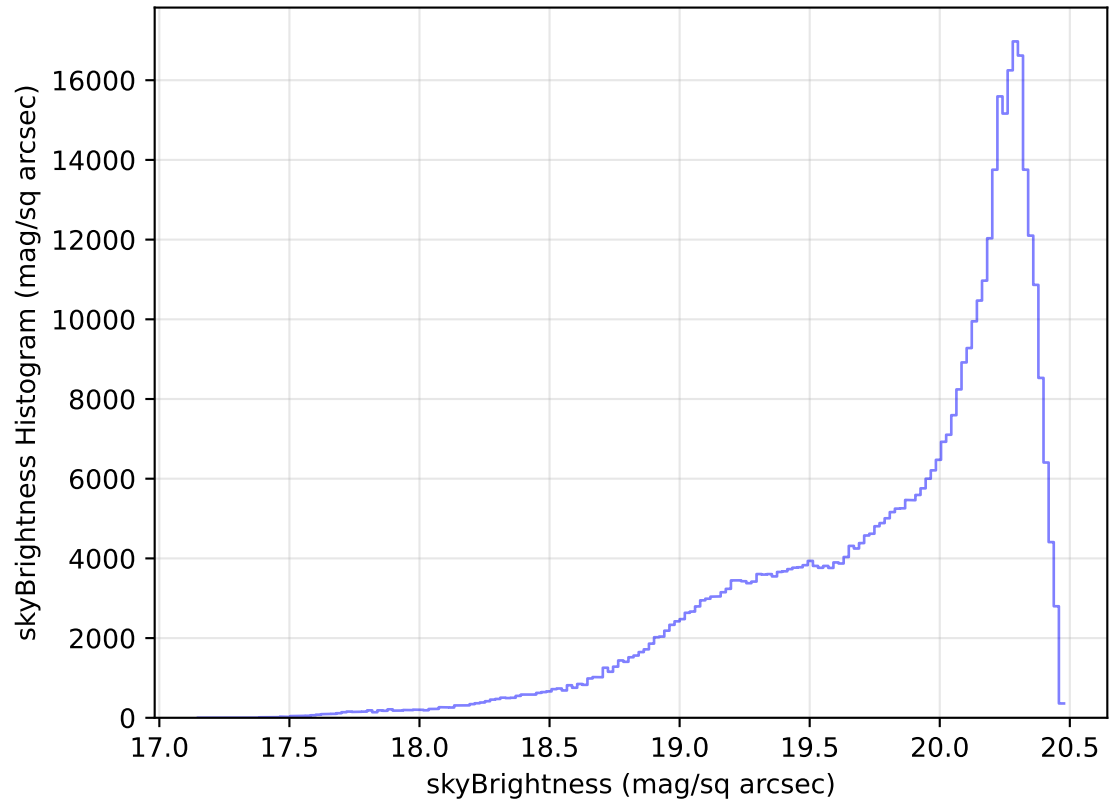
internal_u_expt30_nscale1.0v3.4_10yrs WFD i band: skyBrightness Histogram
