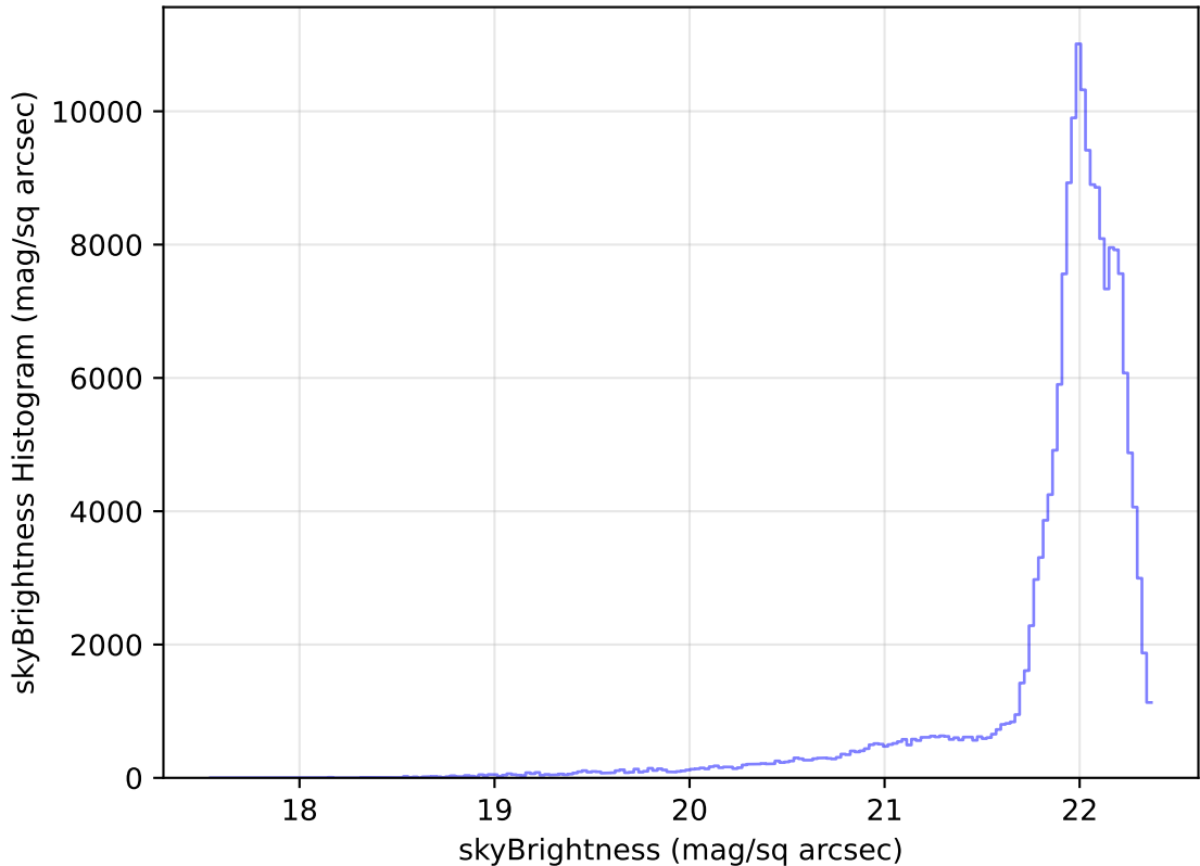
internal_u_expt30_nscale1.0v3.4_10yrs WFD g band: skyBrightness Histogram
