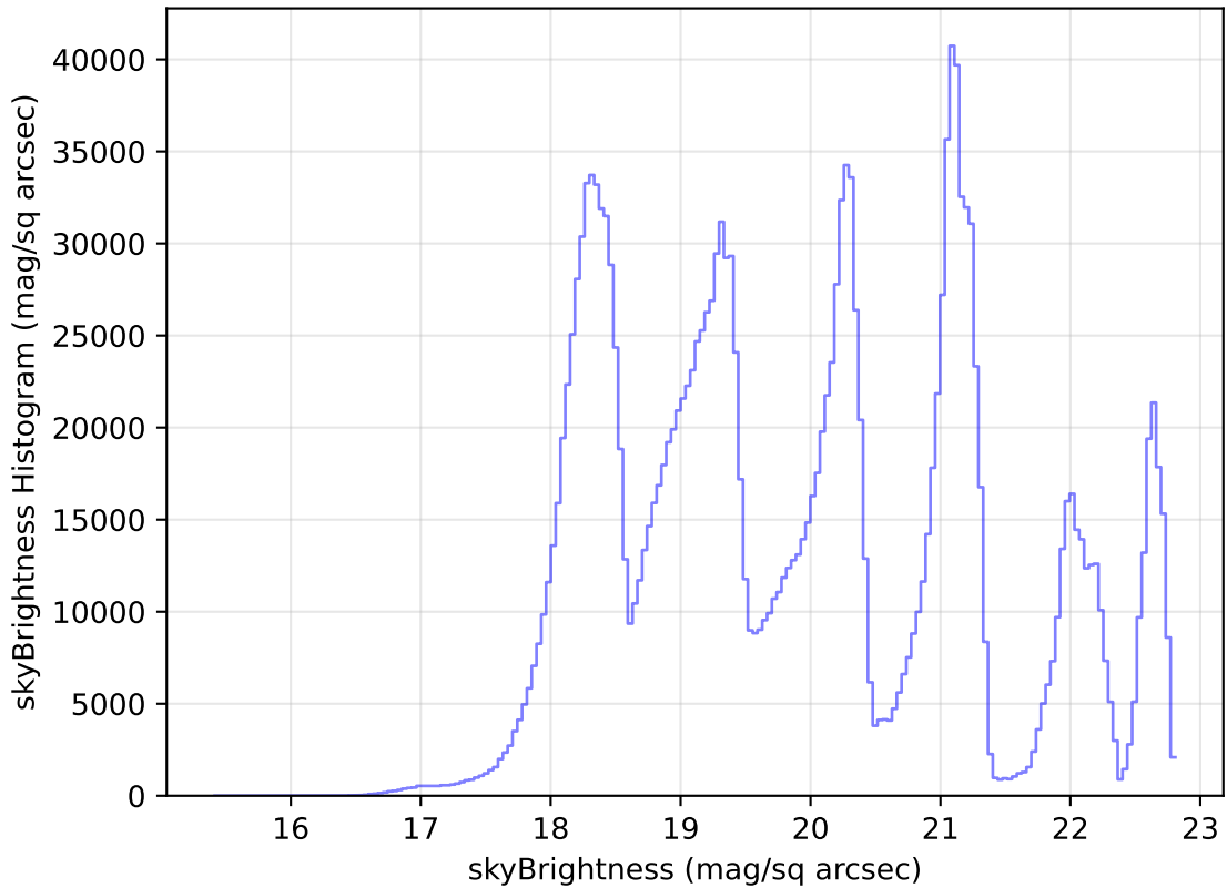
internal_u_expt30_nscale1.0v3.4_10yrs WFD all bands: skyBrightness Histogram
