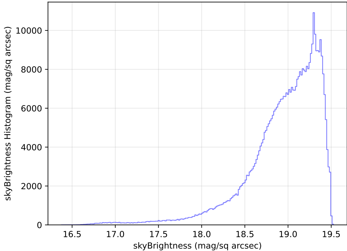
internal_u_expt30_nscale1.0v3.4_10yrs All sky z band: skyBrightness Histogram
