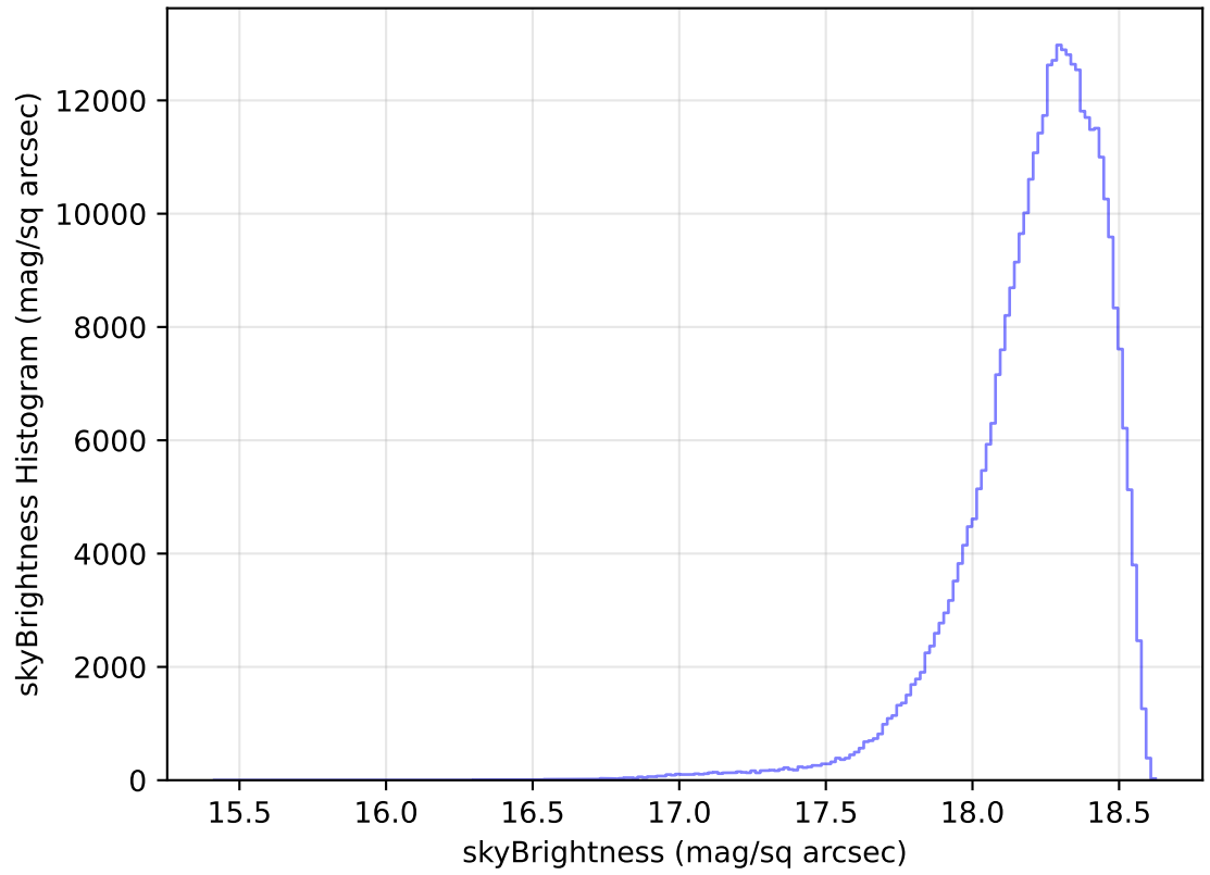
internal_u_expt30_nscale1.0v3.4_10yrs All sky y band: skyBrightness Histogram
