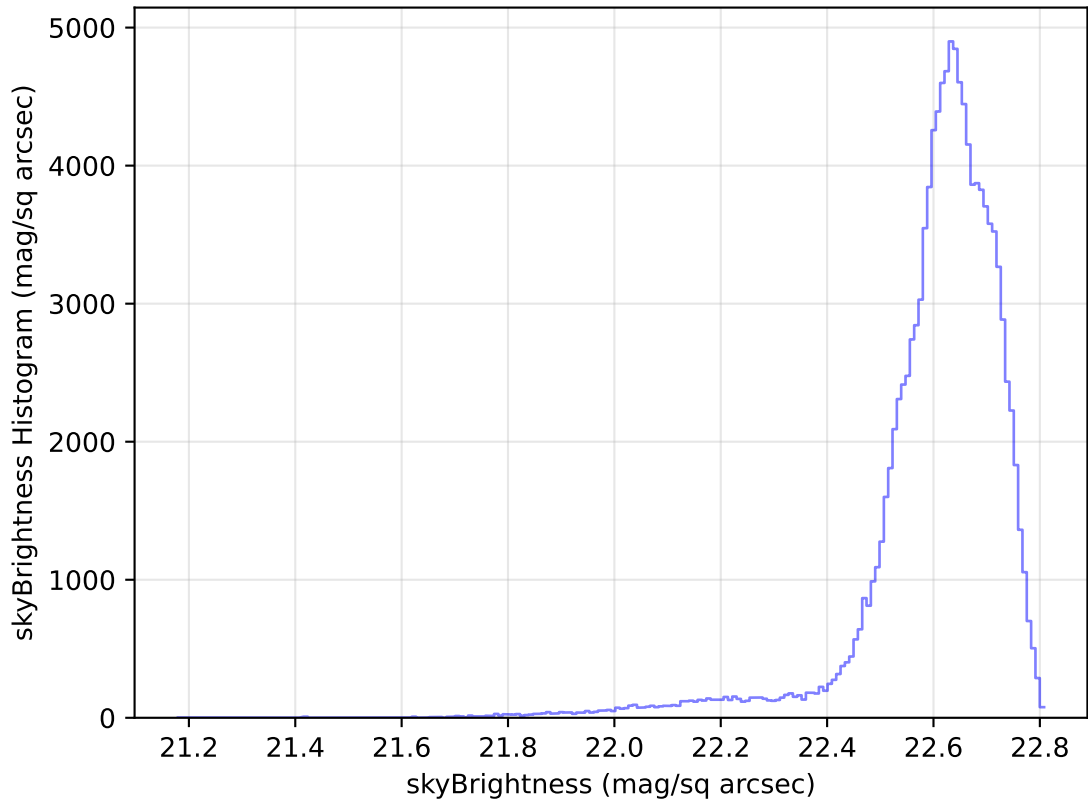
internal_u_expt30_nscale1.0v3.4_10yrs All sky u band: skyBrightness Histogram
