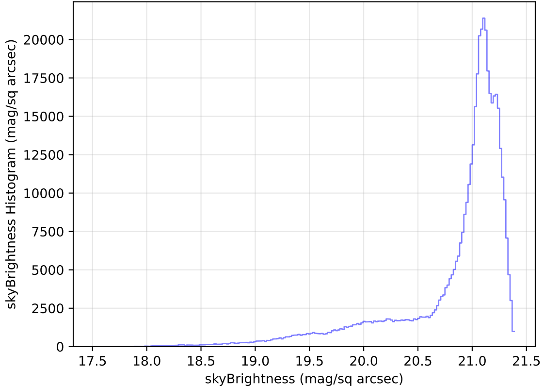
internal_u_expt30_nscale1.0v3.4_10yrs All sky r band: skyBrightness Histogram
