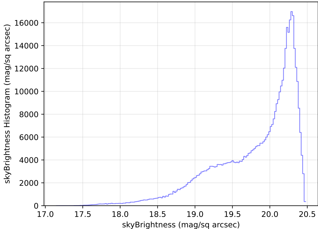
internal_u_expt30_nscale1.0v3.4_10yrs All sky i band: skyBrightness Histogram
