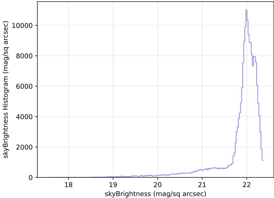
internal_u_expt30_nscale1.0v3.4_10yrs All sky g band: skyBrightness Histogram
