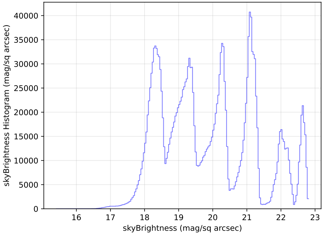
internal_u_expt30_nscale1.0v3.4_10yrs All sky all bands: skyBrightness Histogram
