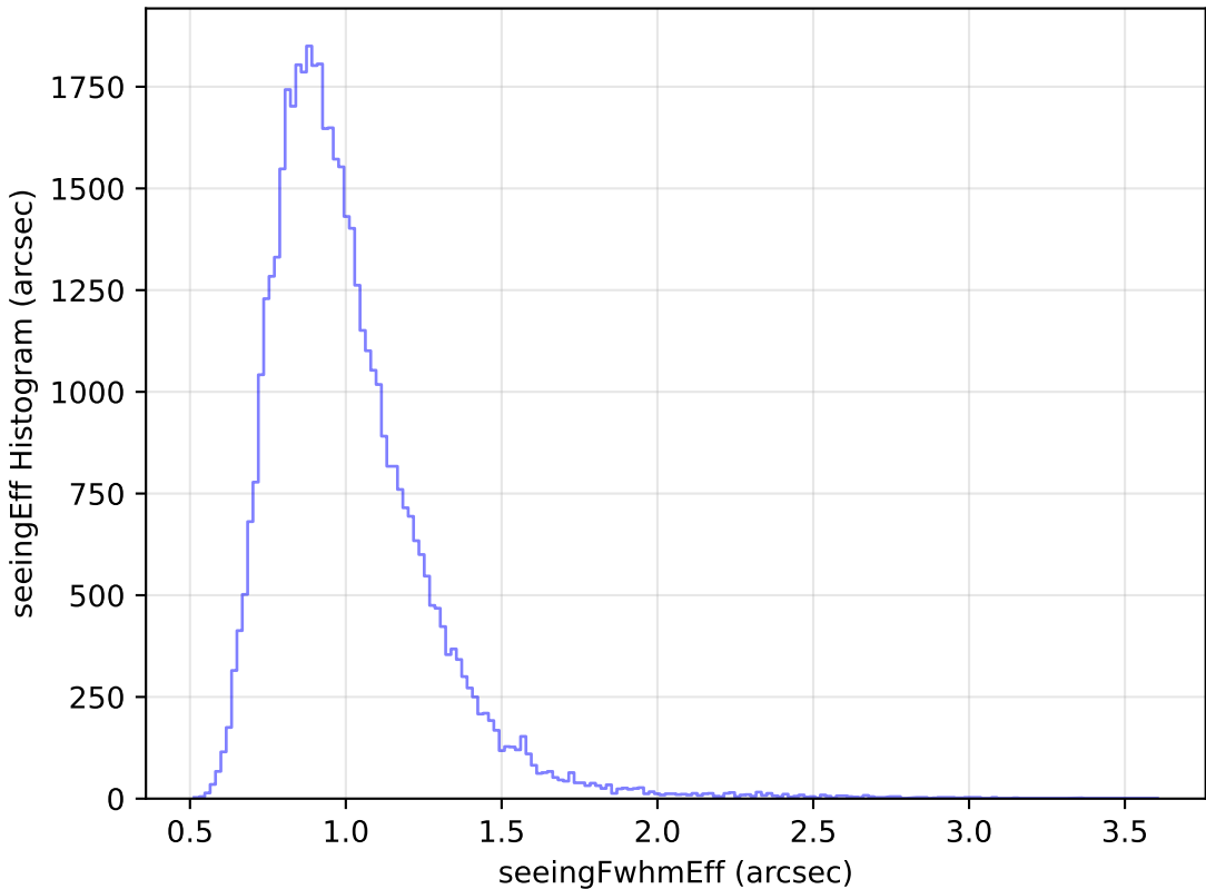
internal_u_expt30_nscale1.0v3.4_10yrs Yr 1 y band: seeingEff Histogram
