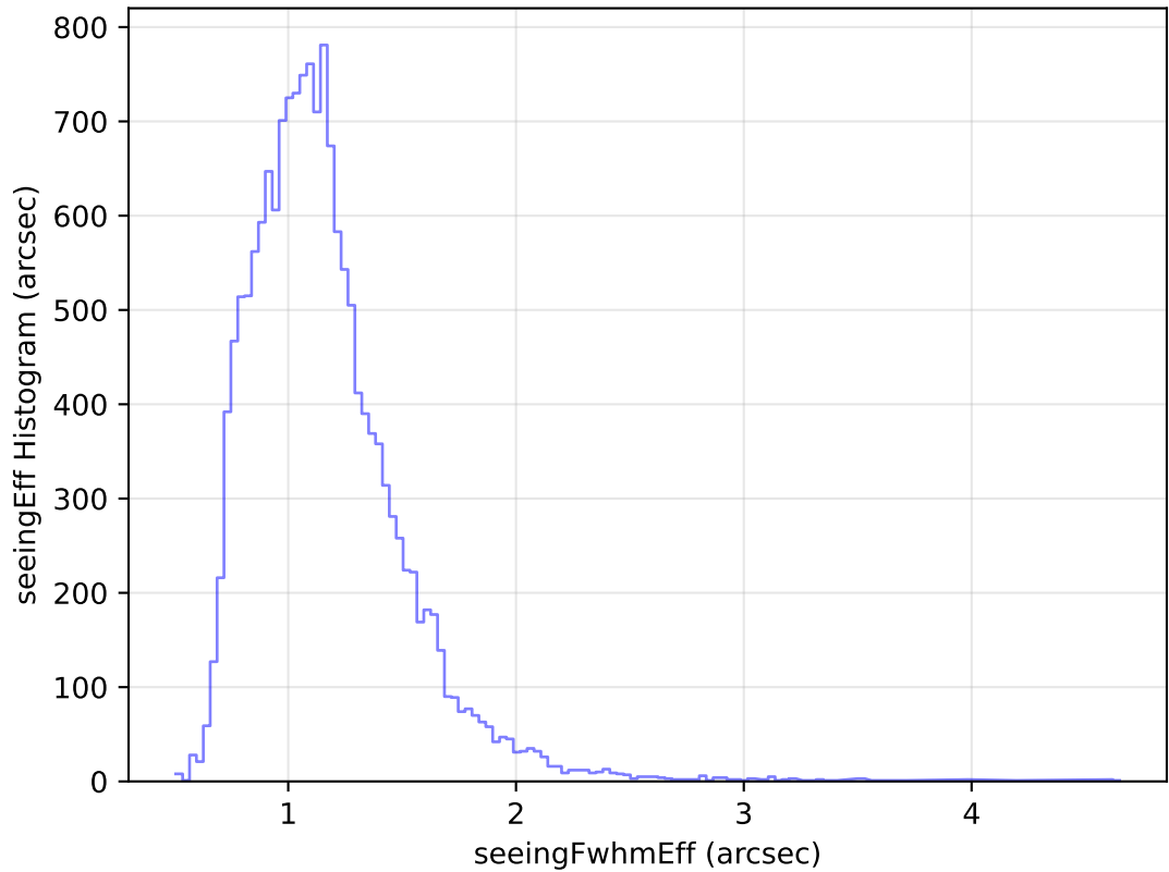
internal_u_expt30_nscale1.0v3.4_10yrs Yr 1 u band: seeingEff Histogram
