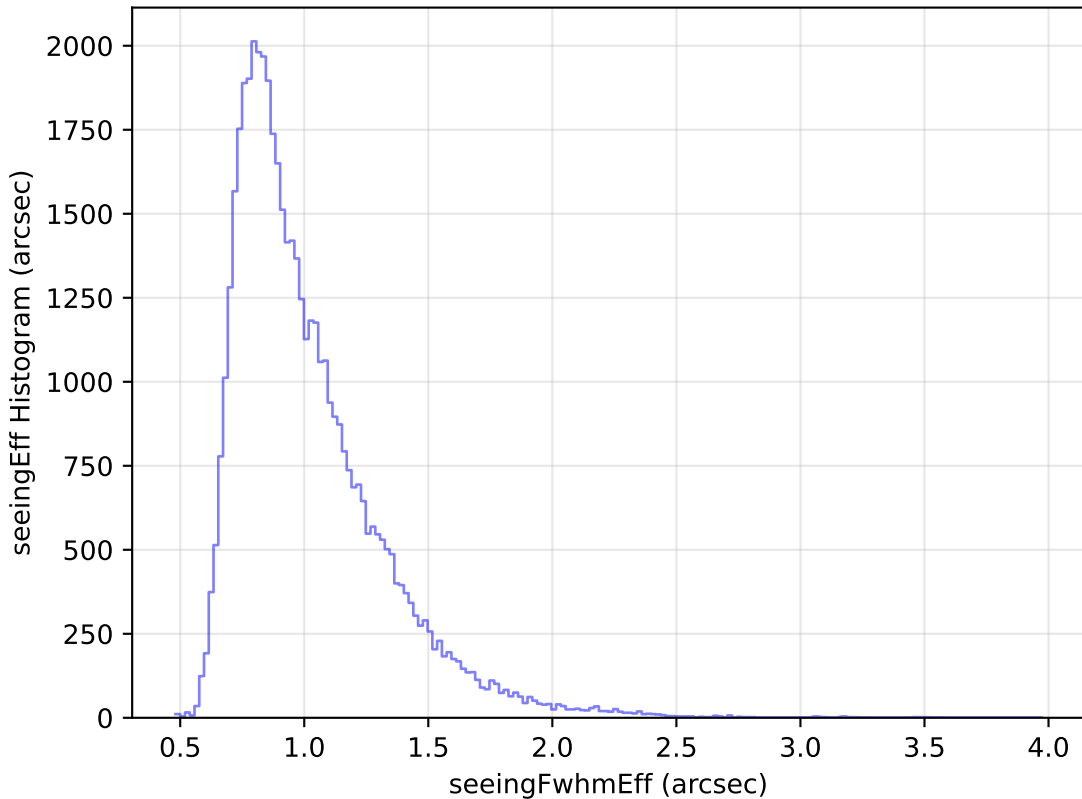
internal_u_expt30_nscale1.0v3.4_10yrs Yr 1 r band: seeingEff Histogram
