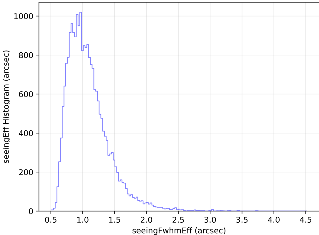
internal_u_expt30_nscale1.0v3.4_10yrs Yr 1 g band: seeingEff Histogram
