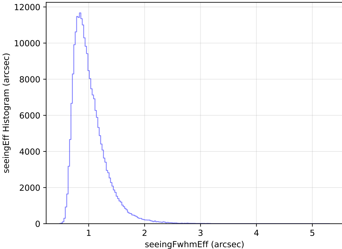
internal_u_expt30_nscale1.0v3.4_10yrs Yr 1 all bands: seeingEff Histogram
