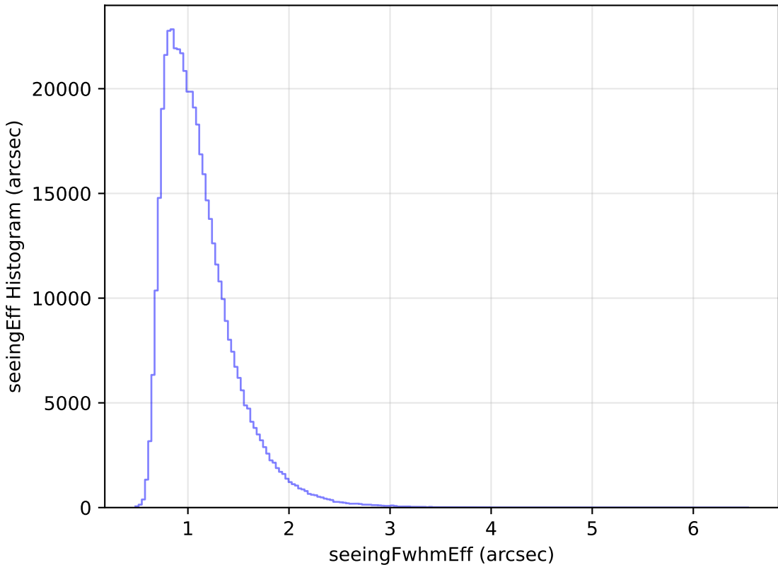
internal_u_expt30_nscale1.0v3.4_10yrs WFD r band: seeingEff Histogram
