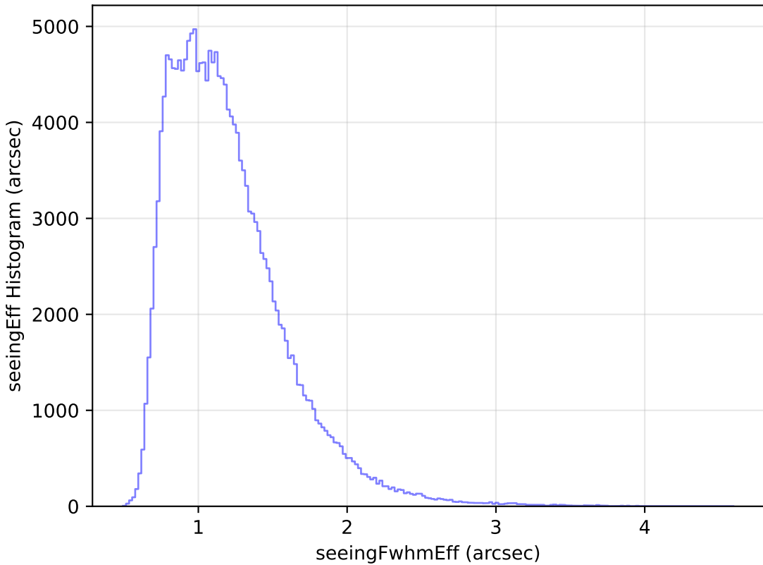
internal_u_expt30_nscale1.0v3.4_10yrs WFD g band: seeingEff Histogram
