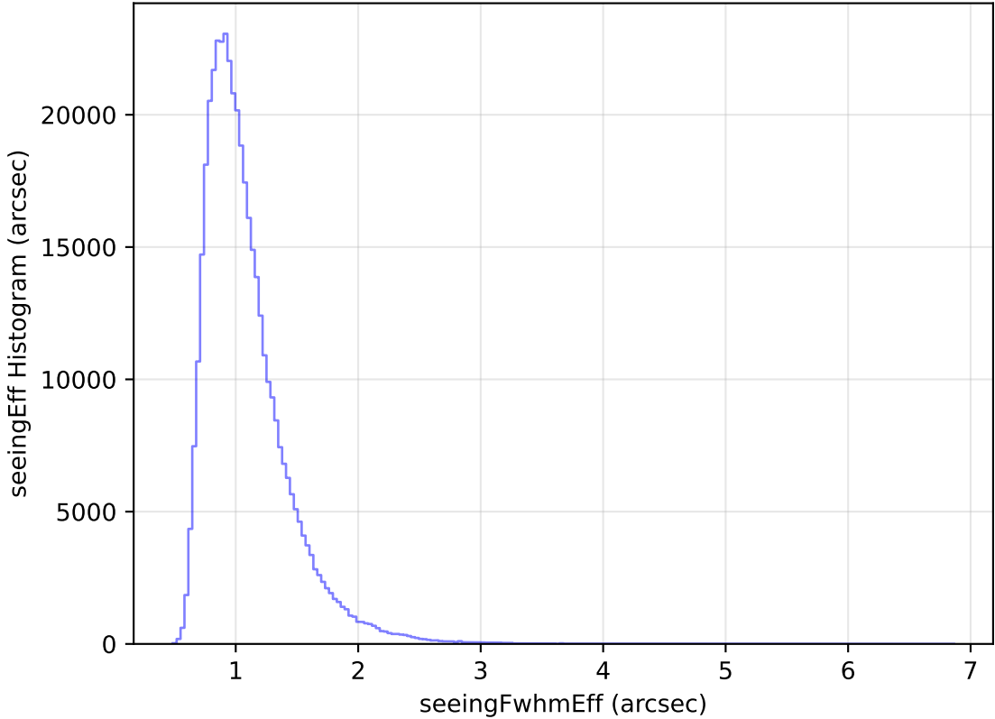
internal_u_expt30_nscale1.0v3.4_10yrs All sky z band: seeingEff Histogram
