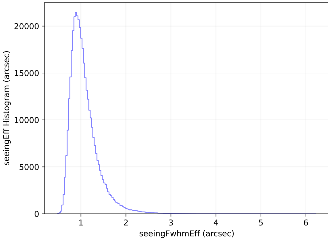
internal_u_expt30_nscale1.0v3.4_10yrs All sky y band: seeingEff Histogram
