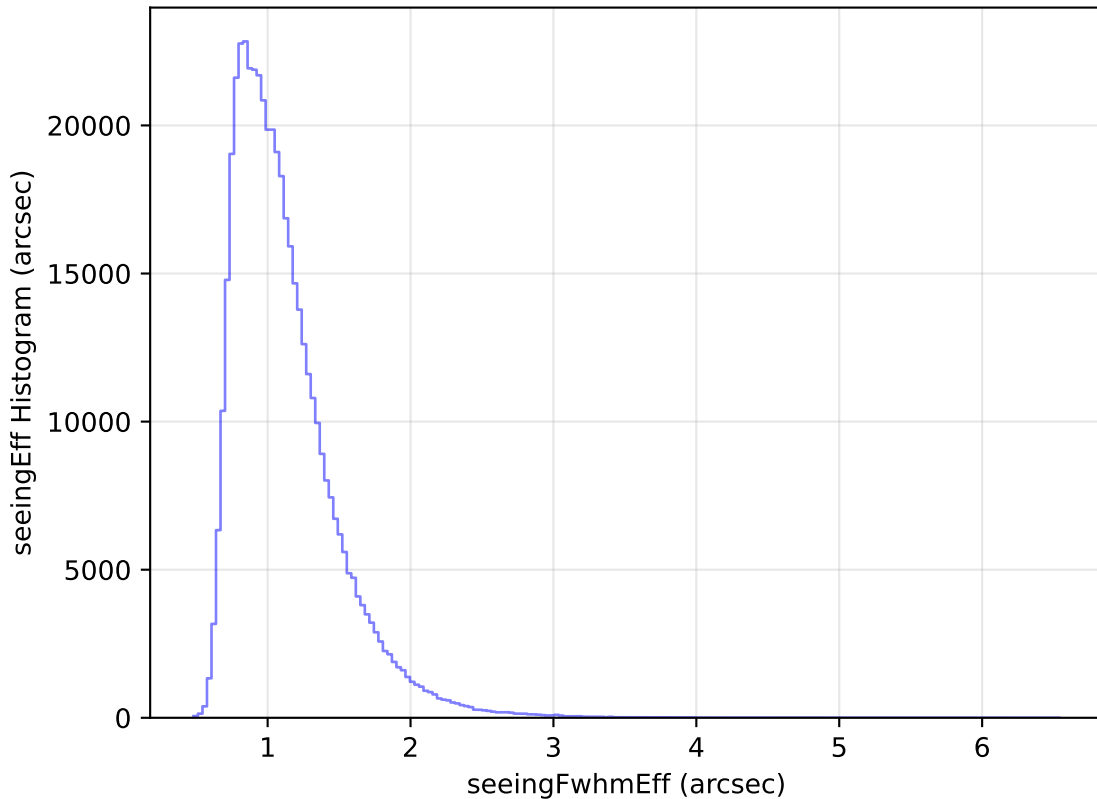
internal_u_expt30_nscale1.0v3.4_10yrs All sky r band: seeingEff Histogram
